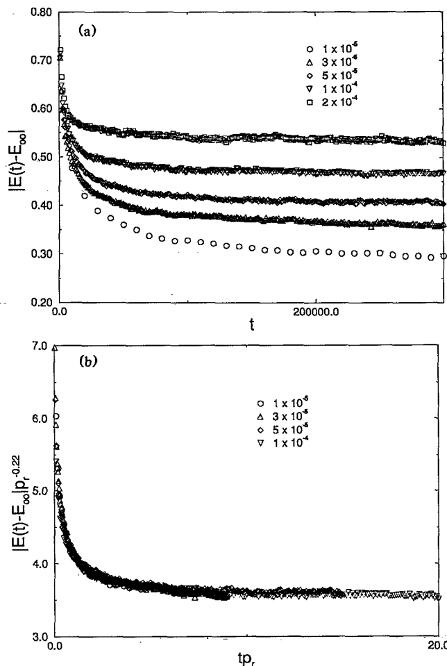
FIG. 3. (a) Energy difference |E(t) - E_{\infty}| vs t for various reaction probabilities p_r , and (b) the data in (a) with the y axis divided by p_r^{0.22} and the x axis multiplied by p_r , to confirm the scaling relation.
