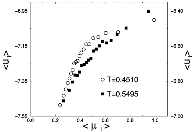
FIG. 15. Potential energy \langle U_i \rangle as a function of the mobility \langle \mu_i \rangle for the A particles. The A particles have been divided into 20 subsets according to their mobility at t^* . Each subset is represented by a point in the graph. The energy scale for T=0.4510 is on the left hand side y axis, while the energy scale for T=0.550 is on the right hand side y axis.
