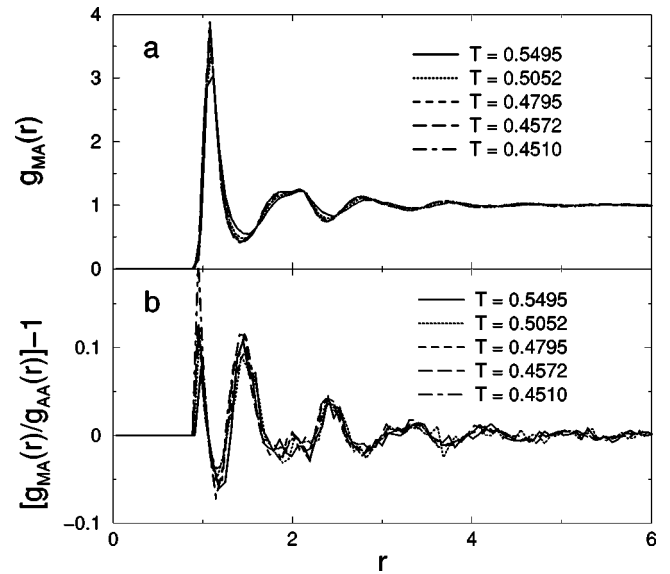
FIG. 16. (a) Pair correlation function g_{MA}(r) between mobile A and generic A particles for several different temperatures. (b) \Gamma(r) = [g_{MA}(r)/g_{AA}(r)] - 1 vs r for several different temperatures.
